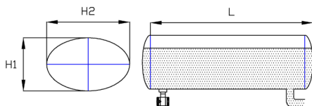
Cylindrical tank with cone-shaped ends
