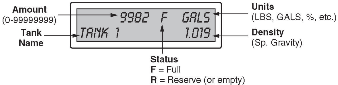
Detail - Tank Level Status Display
