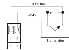
Detail - Onboard 24 Vdc Output
