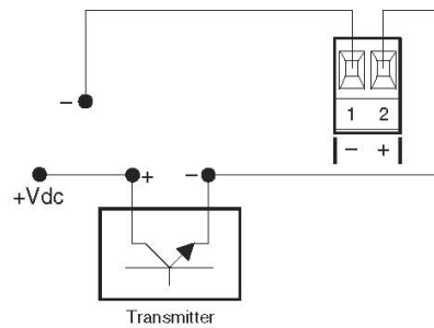
Detail - External Power Supply
